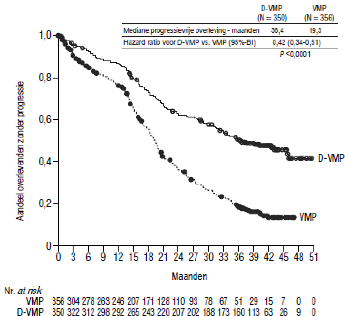
Figuur 4: Kaplan-Meier-curve van PFS in studie MMY3007
