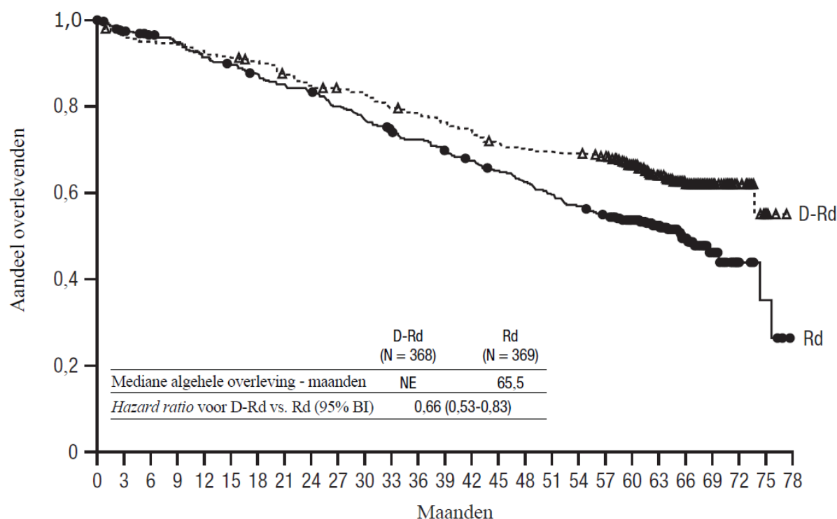
Figuur 3: Kaplan-Meier curve van OS in studie MMY3008
