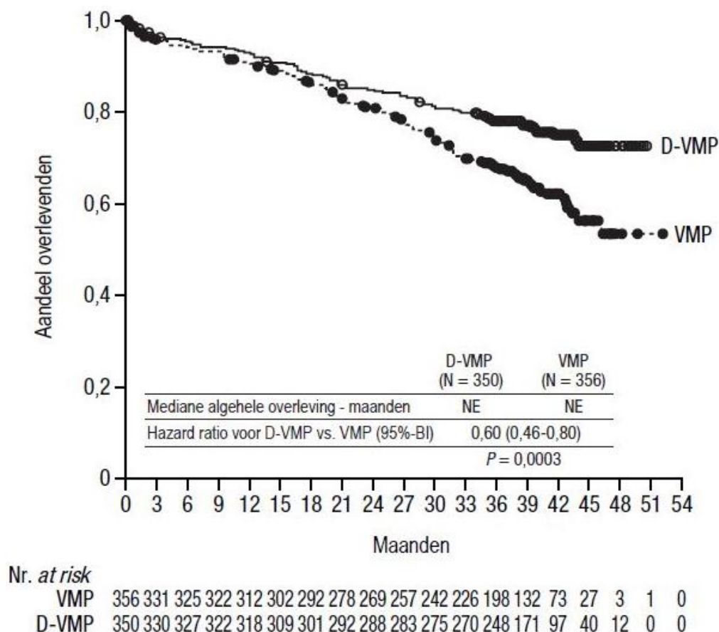
Figuur 5: Kaplan-Meier-curve van OS in studie MMY3007
