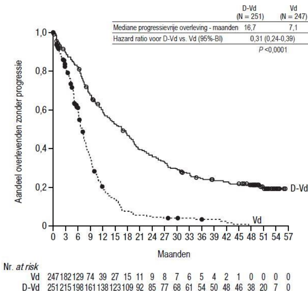
Figuur 8: Kaplan-Meier-curve van progressievrije overleving in studie MMY3004
