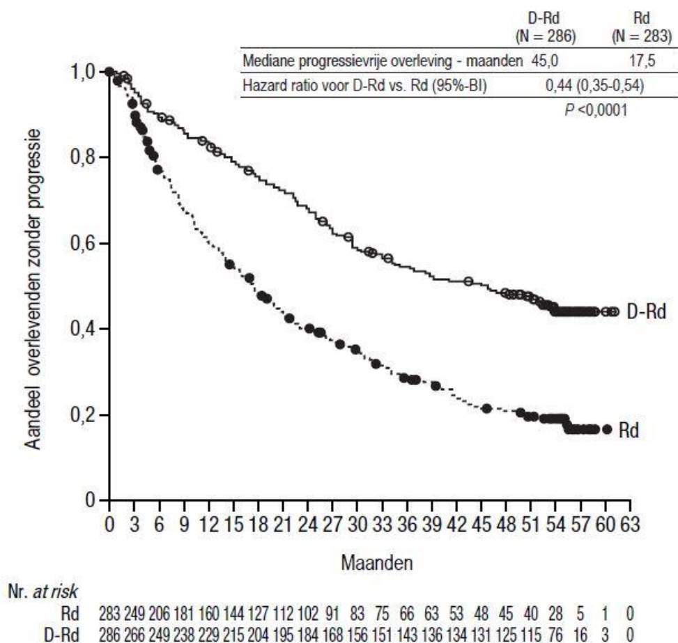
Figuur 7: Kaplan-Meier-curve van progressievrije overleving in studie MMY3003
