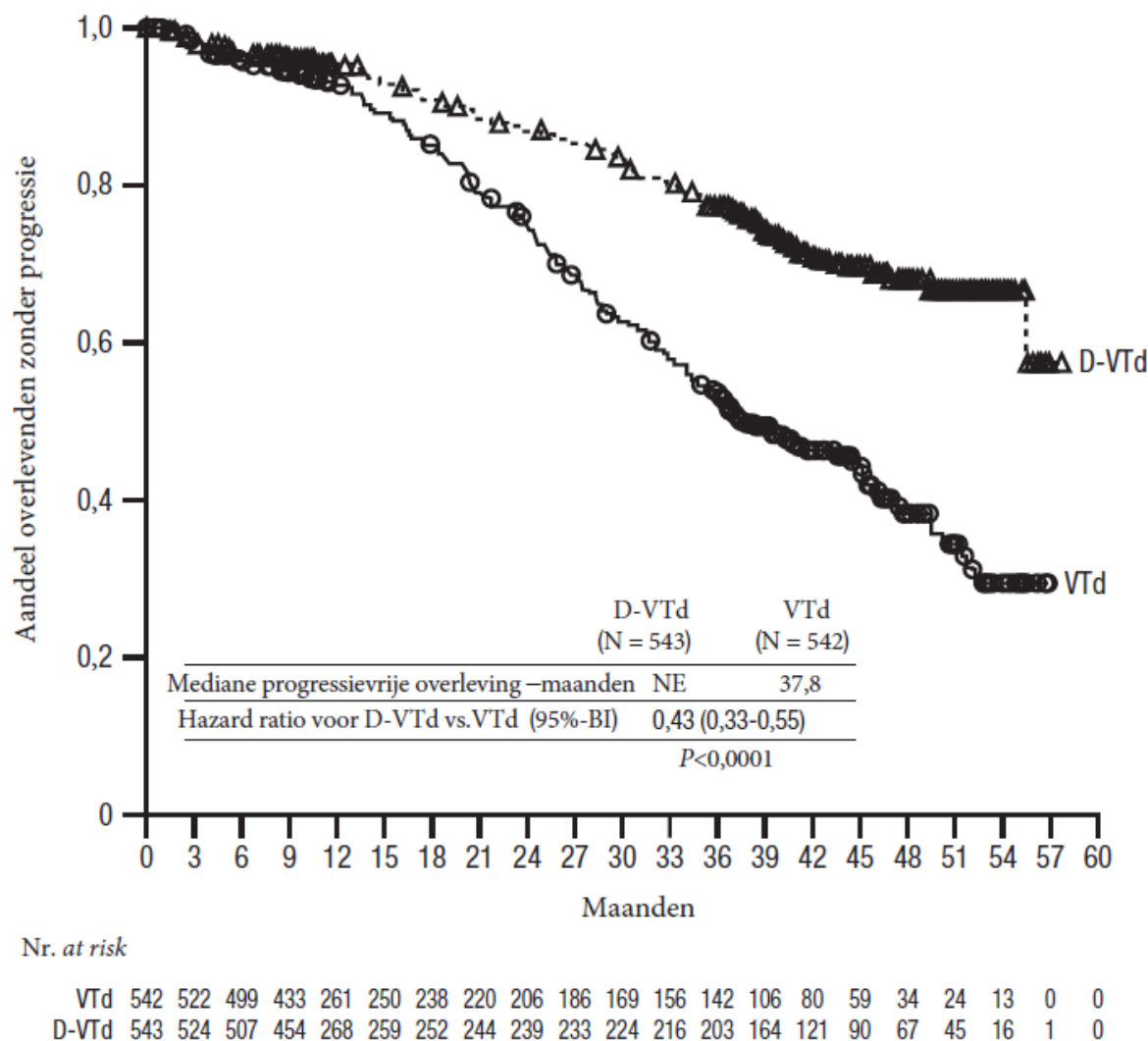
Figuur 6: Kaplan-Meier-curve van PFS in studie MMY3006
