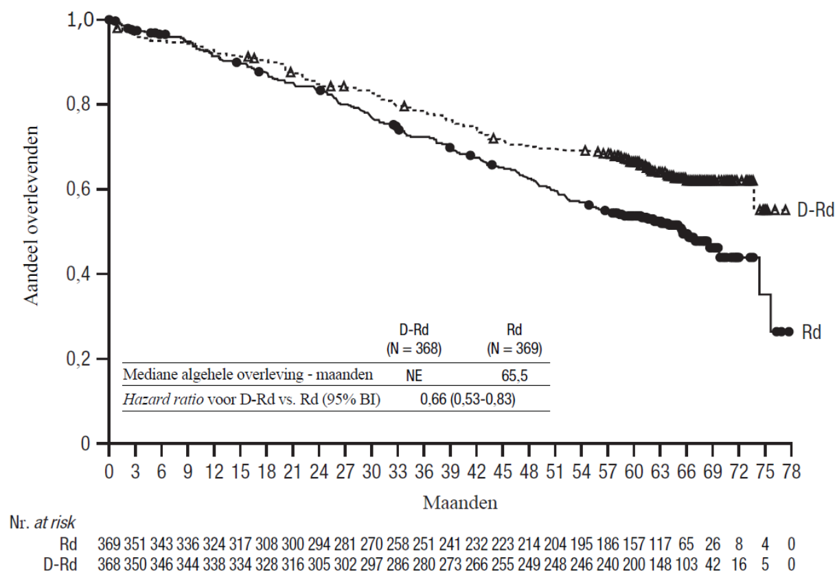
Figuur 2: Kaplan-Meier curve van OS in studie MMY3008
